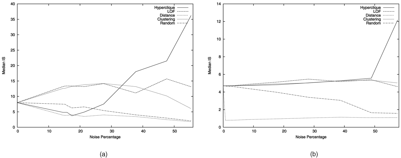
Fig. 13. The impact of noise removal on the results of association analysis for RE0 and OH8 in terms of the IS measure. (a) The RE0 document data set. (b) The OH8 document data set.
