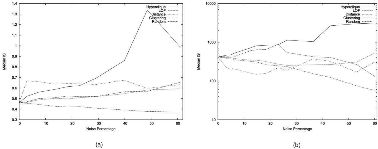
Fig. 12. The impact of noise removal on the results of association analysis for WEST5 and ADS in terms of the IS measure. (a) The WEST5 document data set. (b) The ADS document data set.
