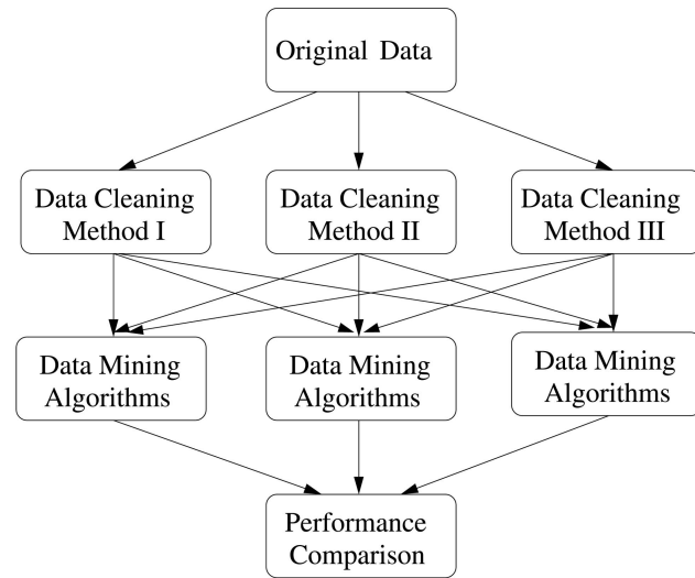
Fig. 6. A data mining framework for validating data cleaning techniques at the data analysis stage.
