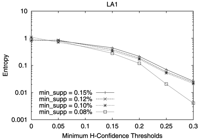
Fig. 4. The cluster nature of hyperclique patterns on the LA1 data set.
