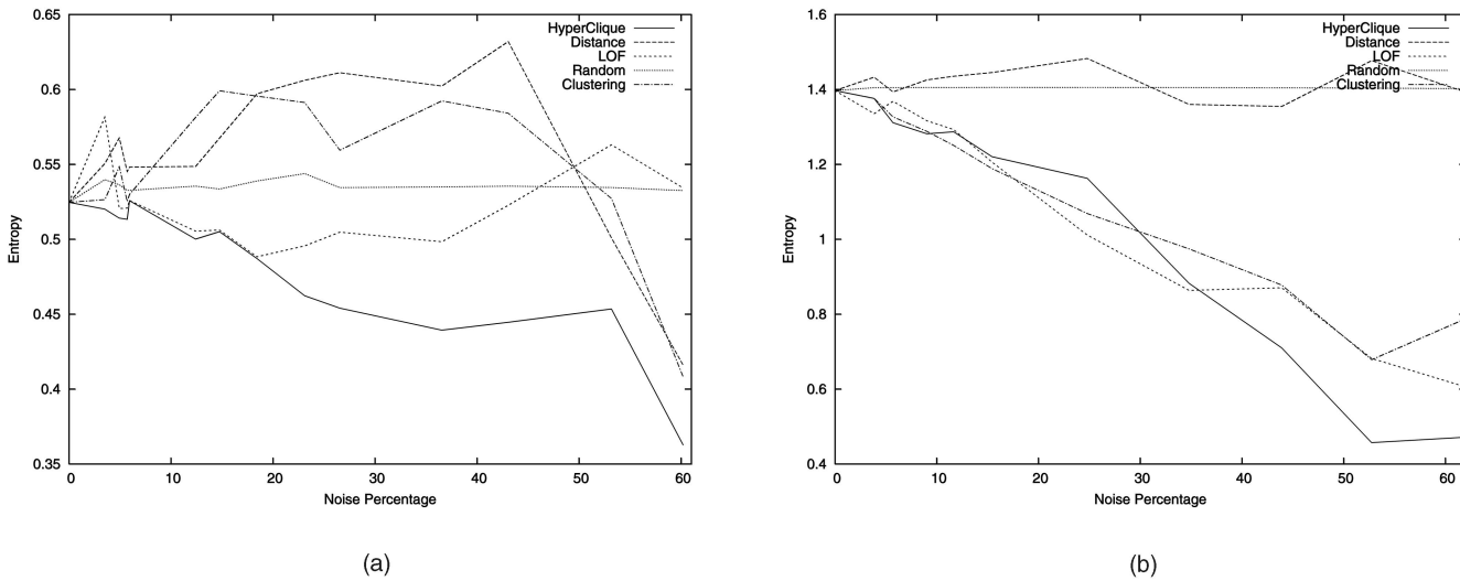
Fig. 8. The impact of noise removal techniques on the performance of clustering analysis for ADS and WAP in terms of entropy. (a) The ADS document data set. (b) The WAP document data set.
