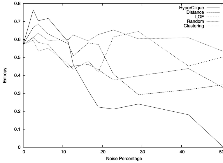
Fig. 10. The impact of noise removal techniques on the performance of clustering analysis for the yeast gene expression data in terms of entropy.
