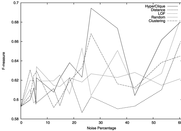
Fig. 11. The impact of noise removal techniques on the performance of clustering analysis for the ADS data set in terms of F-measure.
