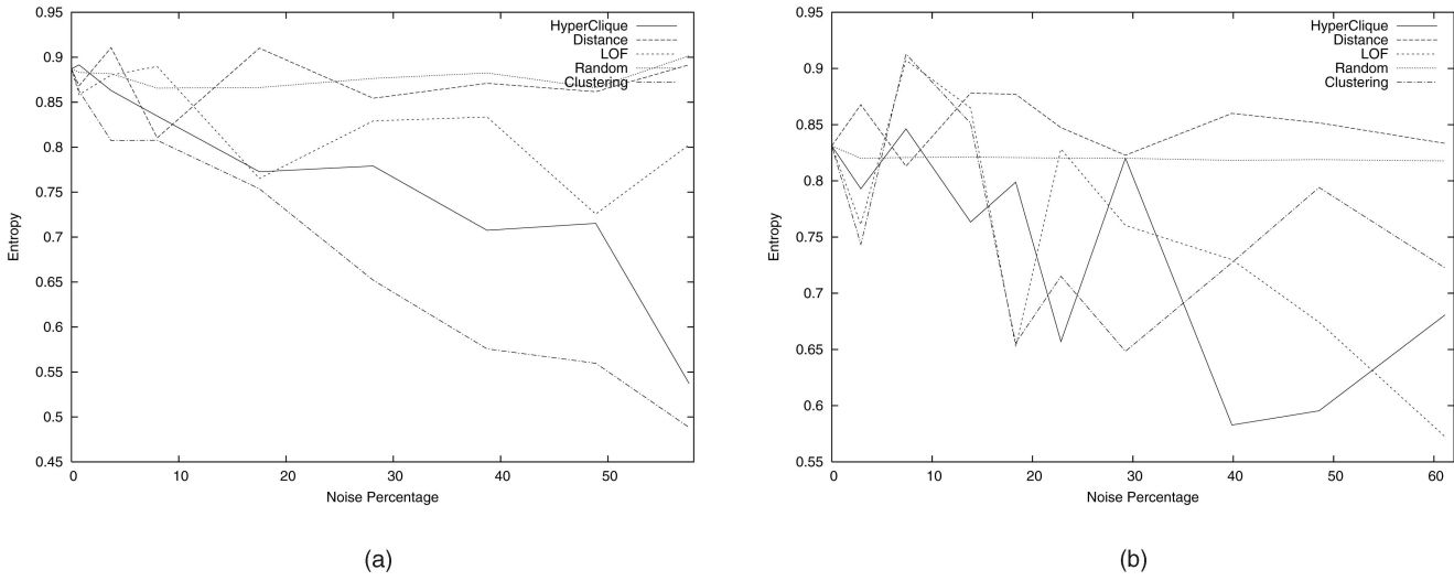
Fig. 9. The impact of noise removal techniques on the performance of clustering analysis for OH8 and WEST5 in terms of entropy. (a) The OH8 data set. (b) The WEST5 data set.
