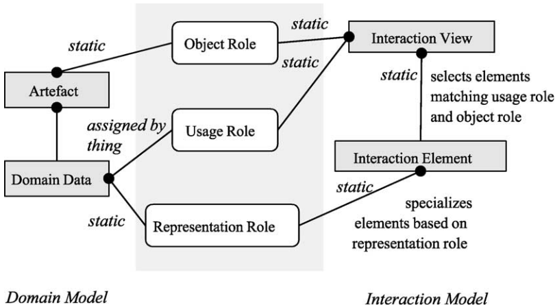
Fig. 7. Relationship between domain objects and interaction objects.
