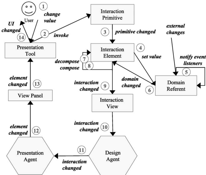
Fig. 9. MAID communication paradigm.
