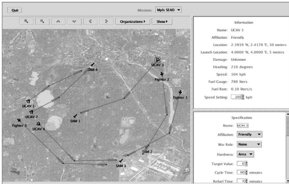
Fig. 2. Example AID-generated user interface.
