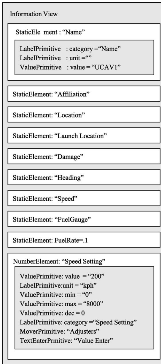
Fig. 6. Example interaction design for an Information View referencing a UAV.
