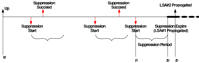
Fig. 6. Link events and effects with suppression
