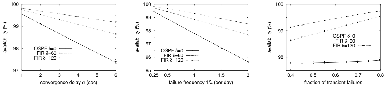
Fig. 12. Simulation results under various settings: (a) convergence delay; (b) failure frequency; (c) transient failures
