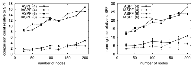
Fig. 13. Complexity of FIR: (a) comparisons; (b) running time
