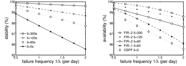
Fig. 7. Impact of failure frequency on network: (a) stability; (b) availability.
