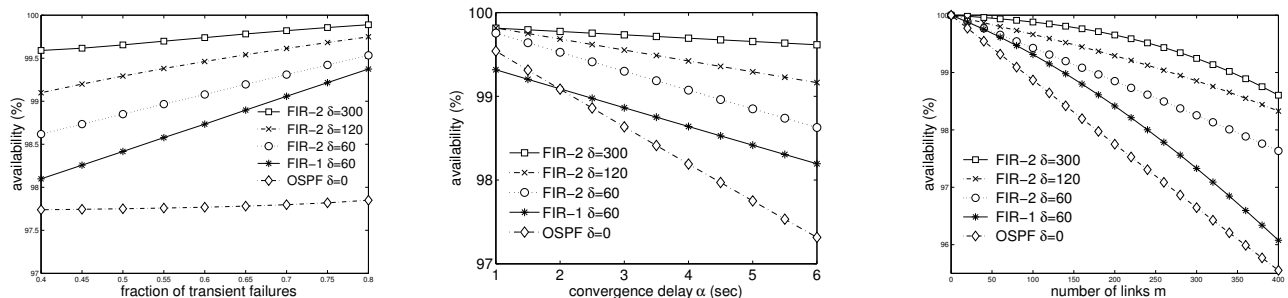
Fig. 9. Network availability under various settings: (a) transient failures; (b) convergence delay (c) network size.
